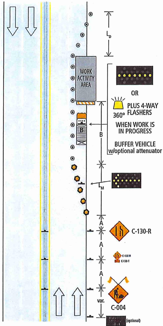
Figure 9.6: Right Lane Closed - Short Duration - Multi-Lane Roadway
